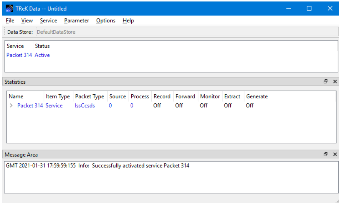
Figure 45 Packet 314 Activated
