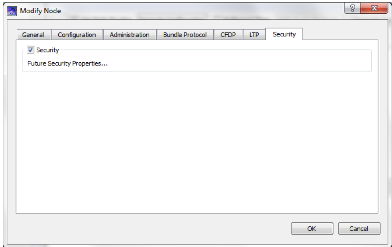
Figure 19 Security Properties
