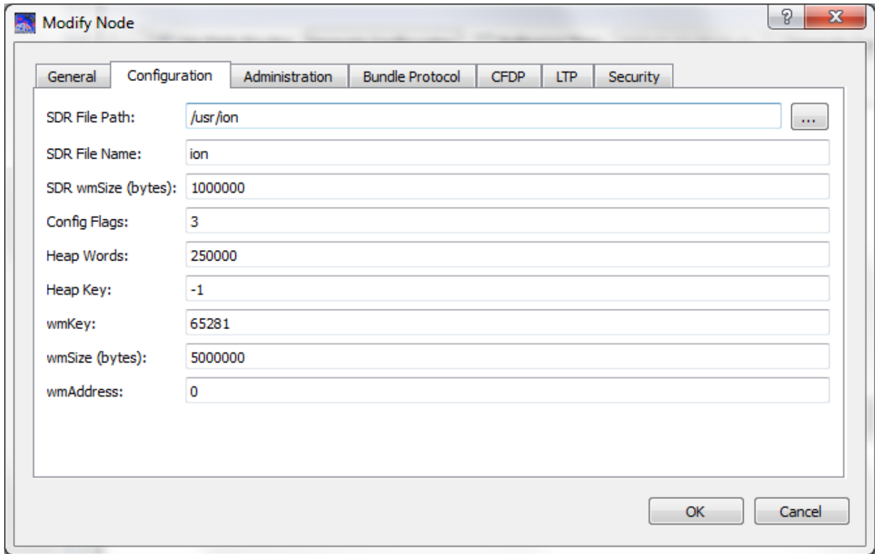
Figure 12 Configuration Properties
