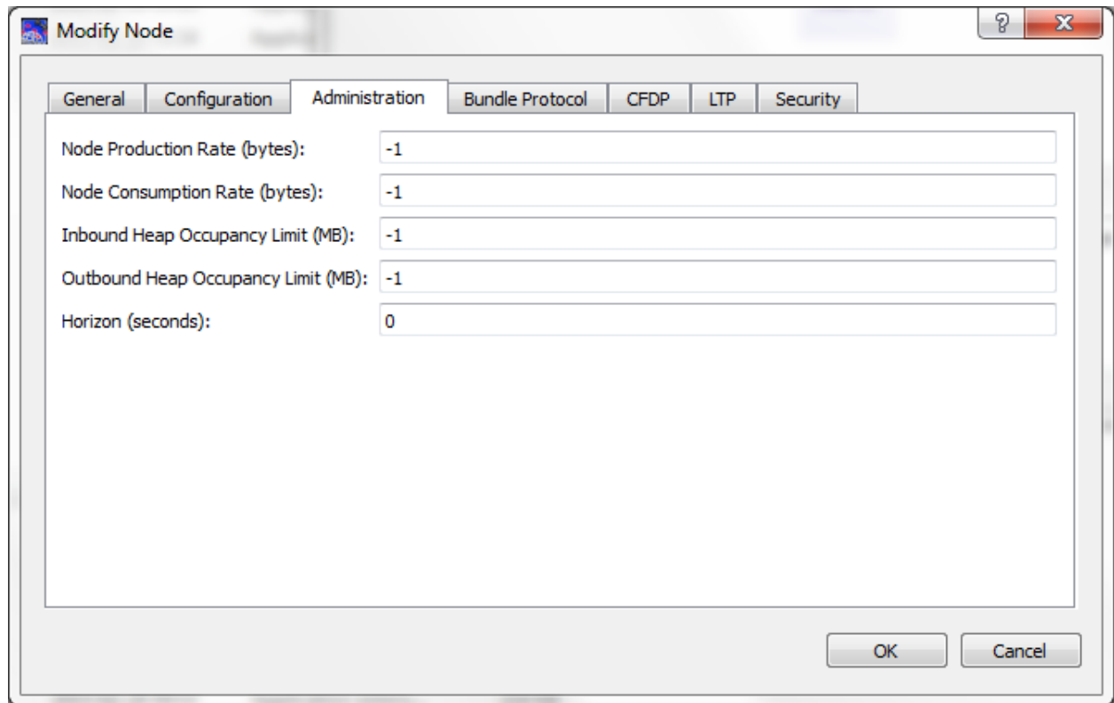
Figure 14 Administration Properties
