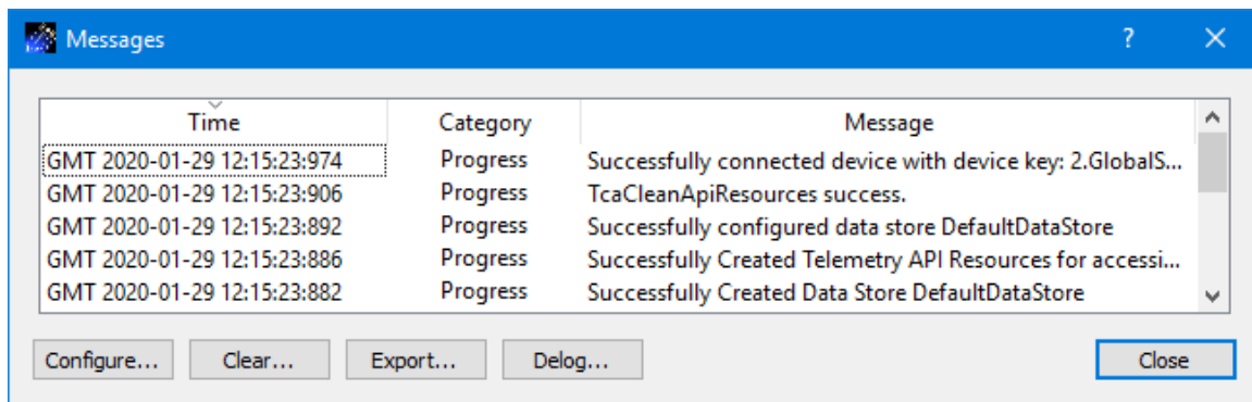
Figure 98 Messages Dialog
