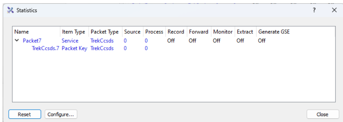
Figure 67 Statistics Dialog
