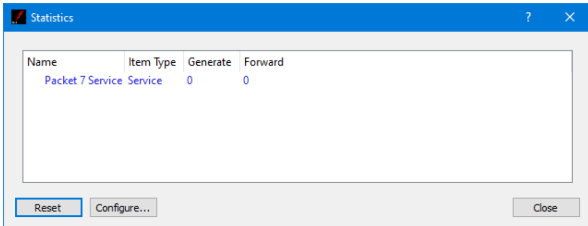
Figure 14 Statistics Dialog
