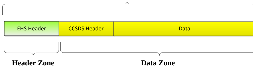
PDSS Payload Packet with EHS Header and Data Zone containing CCSDS Packet
