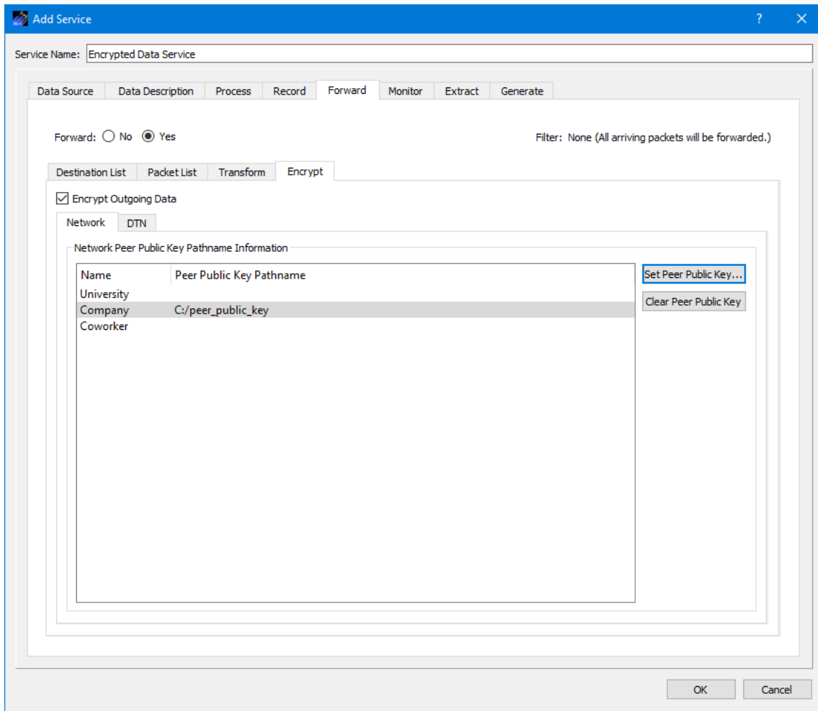
Figure 15 TReK Data Forward Tab Encrypt Tab
