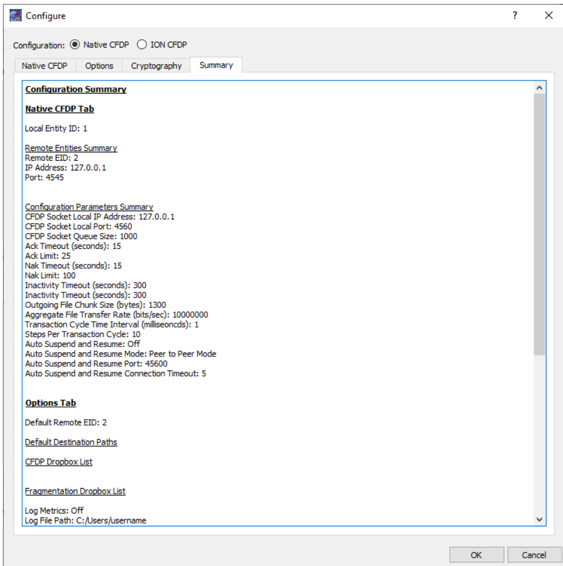
Figure 12 Summary Tab
