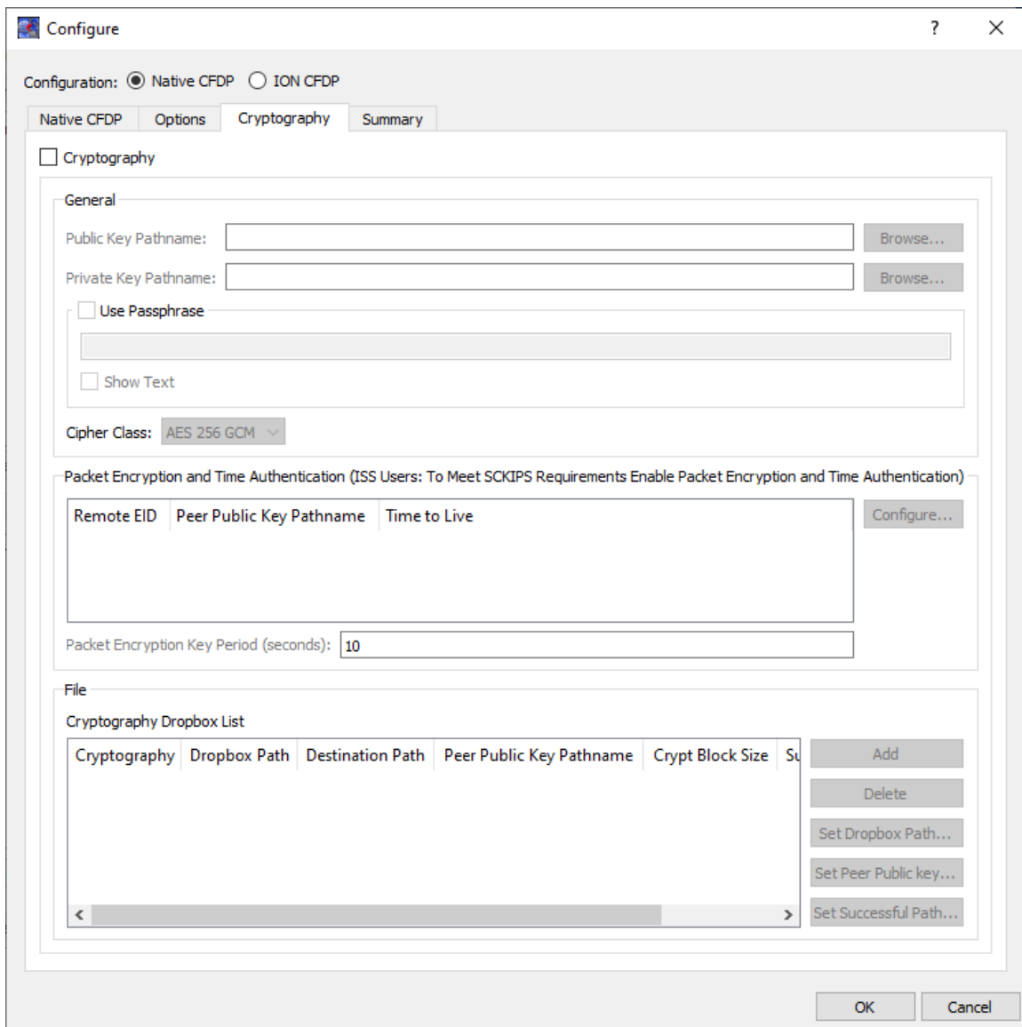
Figure 6 Configure Dialog (Cryptography Tab)
