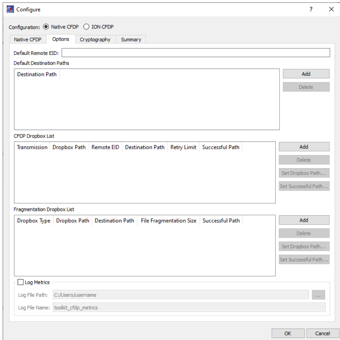
Figure 5 Configure Dialog (Options Tab)
