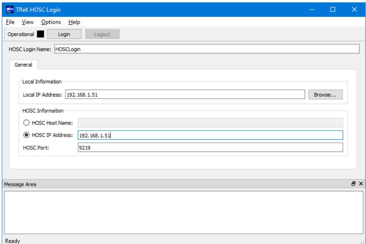
Figure 1 Main Window
